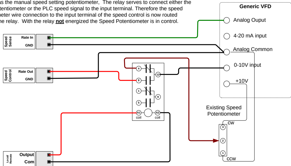
Figure 51 - DM510 to Generic VFD (0-10 vdc)
