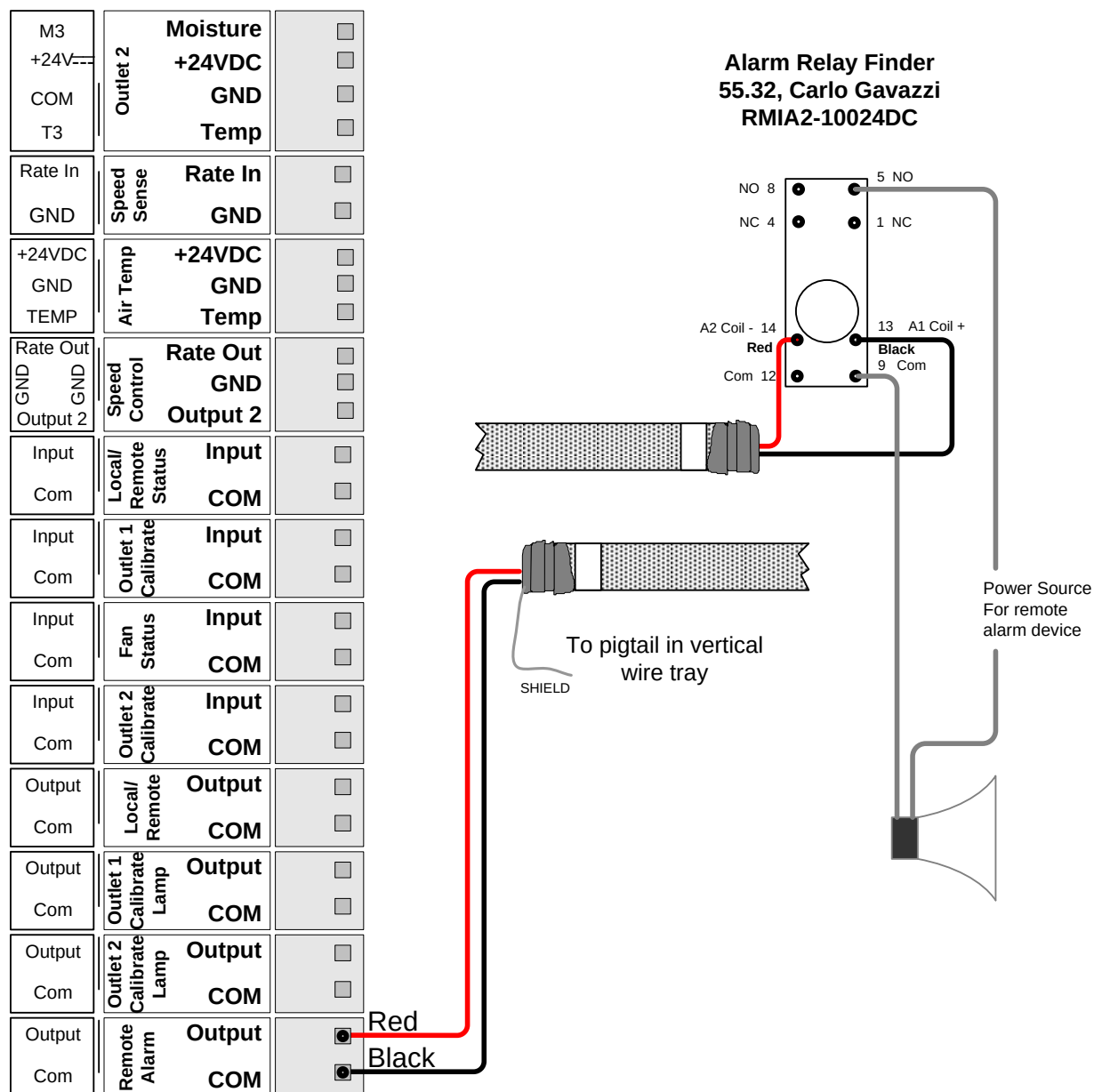
Figure 49 - Remote Alarm
