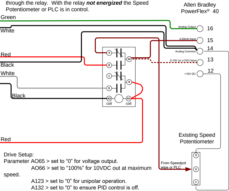
Figure 52 - DM510 to Allen Bradley PowerFlex40
